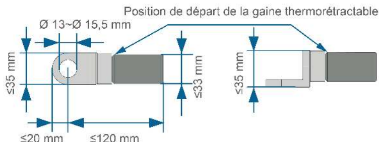
figure 5-5 Spécifications des bornes OT/DT series
