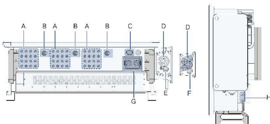
figure 5-1 Description des bornes (SG125/110CX-P2)
