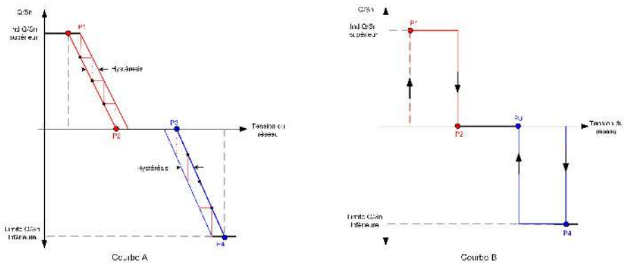
figure 7-19 Courbe Q(U)
